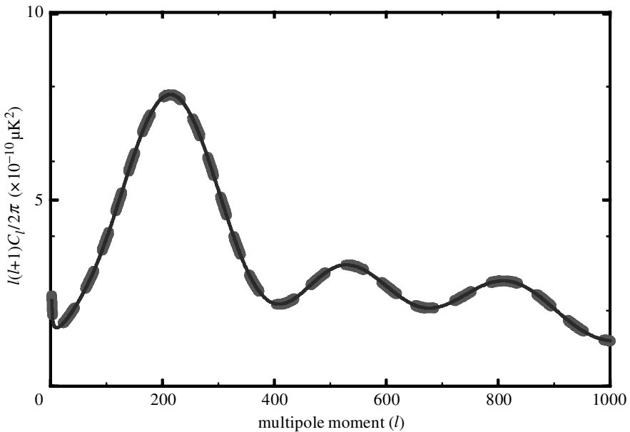
Figure 3. An illustration of the CMB degeneracy problem: the CMB power spectra completely overlap for a flat quintessence model with w = -0.56 , \Omega_m = 0.30 , \Omega_Q = 0.7 , and h = 0.56 (thick dashed line) and a closed model with w = -1 , \Omega_m = 0.35 , \Omega_\Lambda = 0.7 and h = 0.6 (thin solid line).
